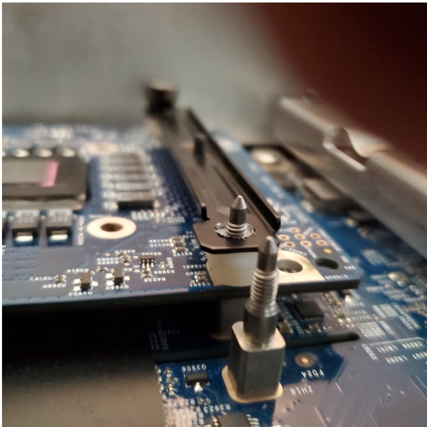
Front mounting hardware sitting on the alignment pegs Photo courtesy of MacRumors user Amishallan
