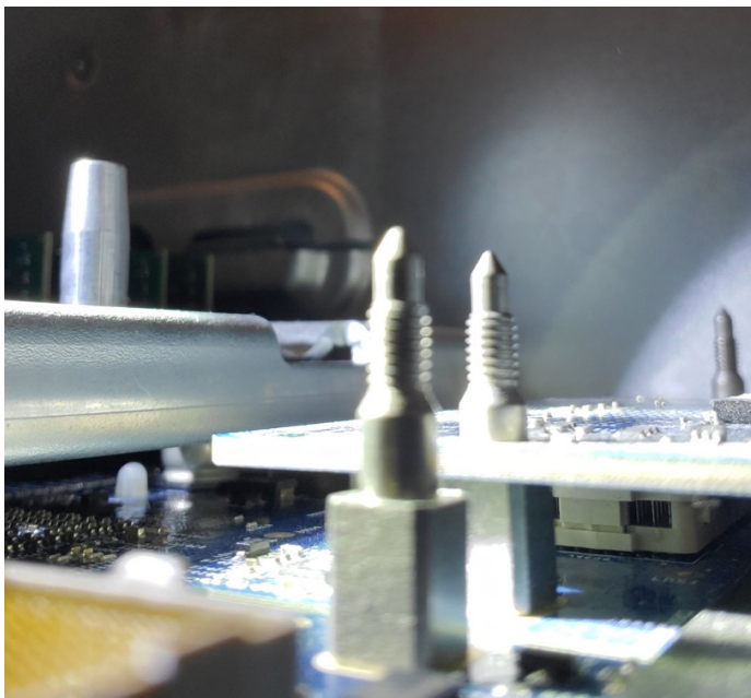
Motherboard mounting/alignment pegs Photo courtesy of MacRumors user Amishallan
