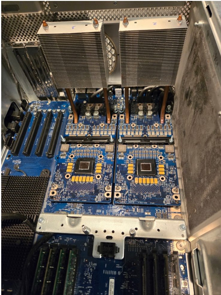
CPU cards, back mounting hardware in place
